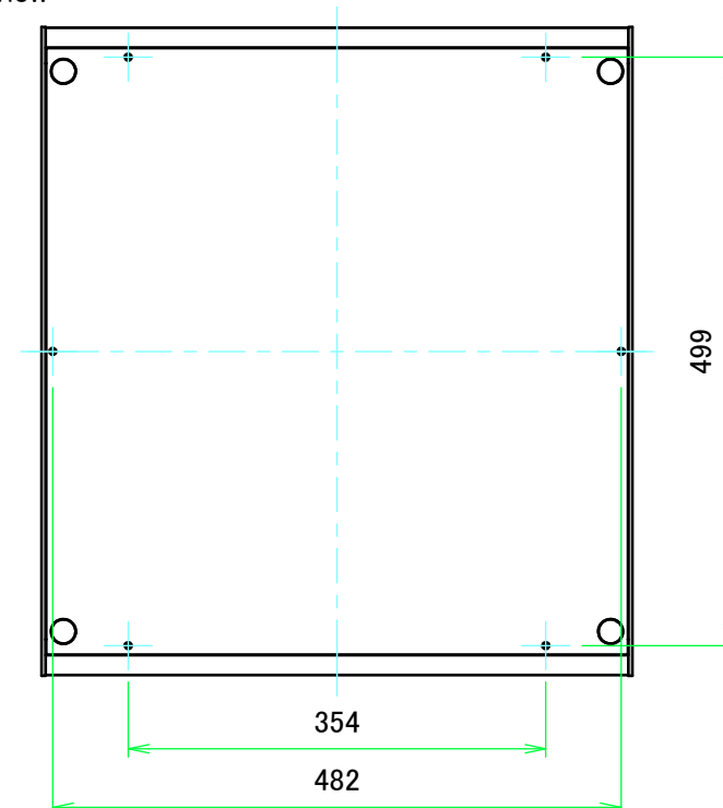
F view
