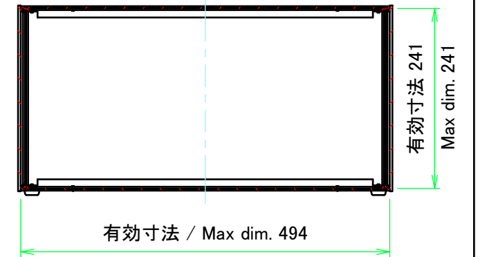
C-C (1:7)
