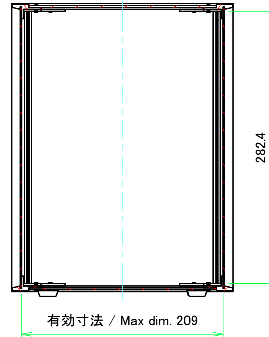
C view
