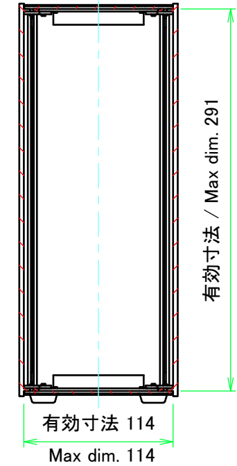
B view
