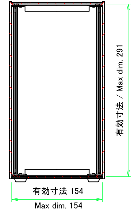
B view
