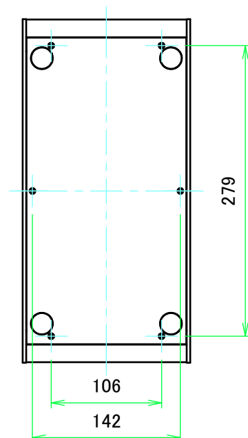
F view
