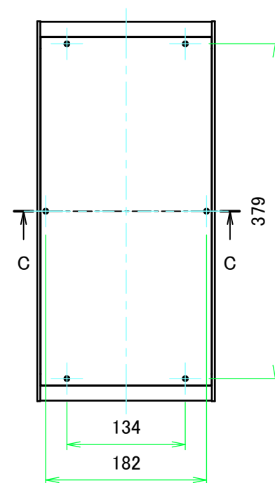
E view
