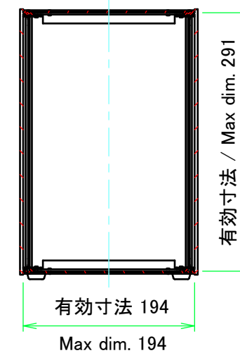
C-C (1:6)
