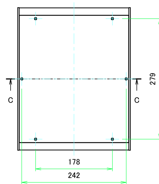
E view
