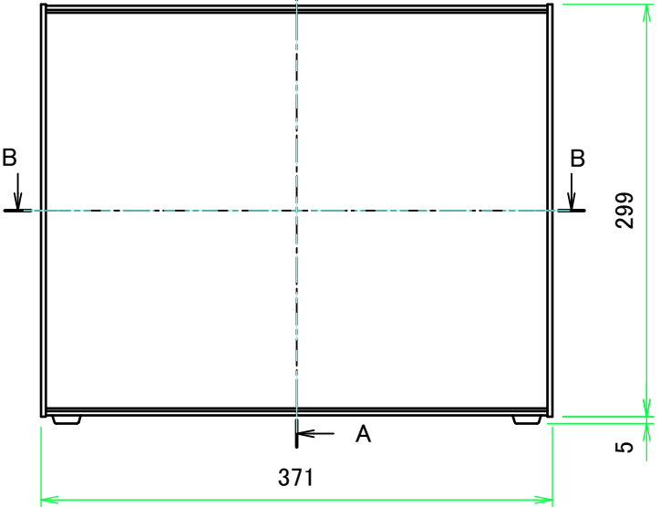
F view
