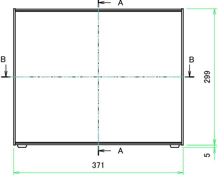
F view
