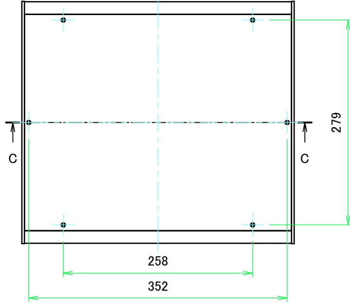
A view
