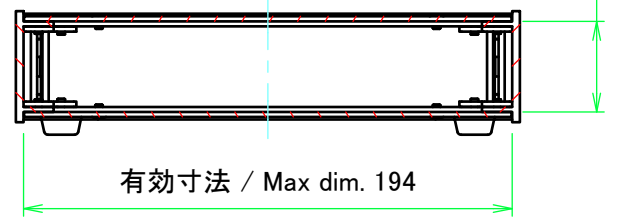
C-C (1:3)
