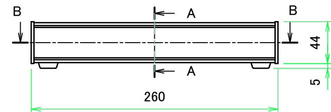
F view
