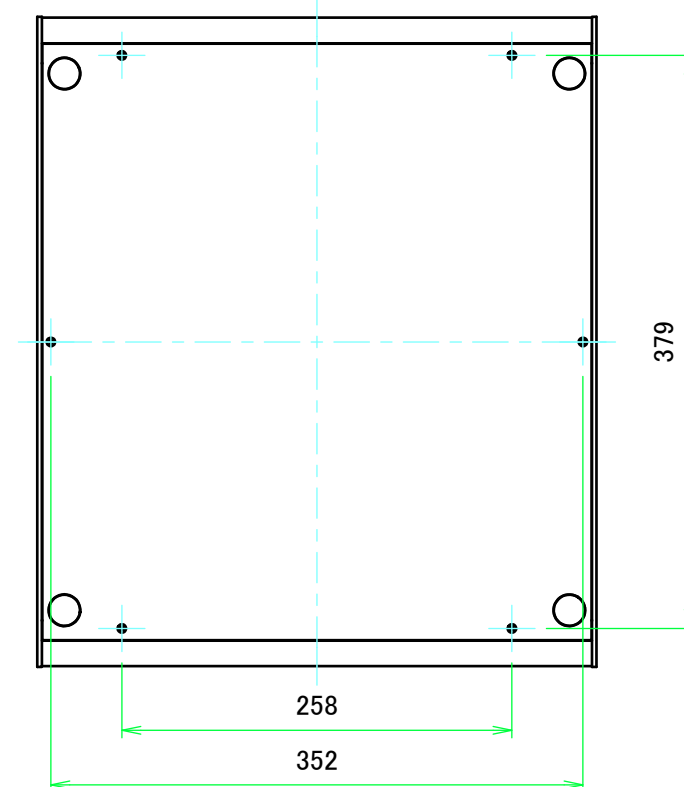
F view
