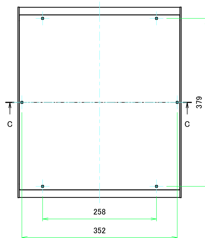
A view
