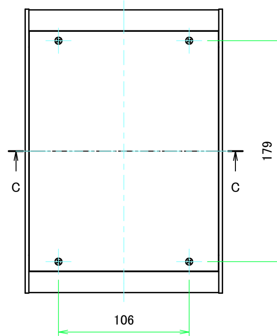
E view
