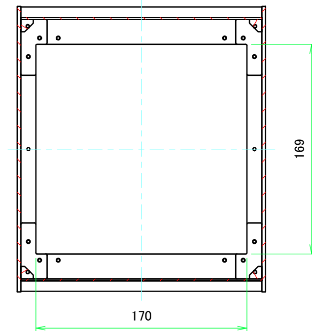
B-B (1:3)
