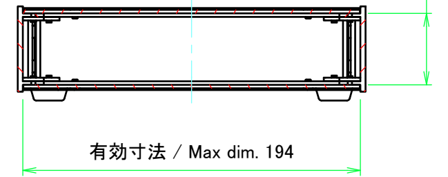
C-C (1:3)
