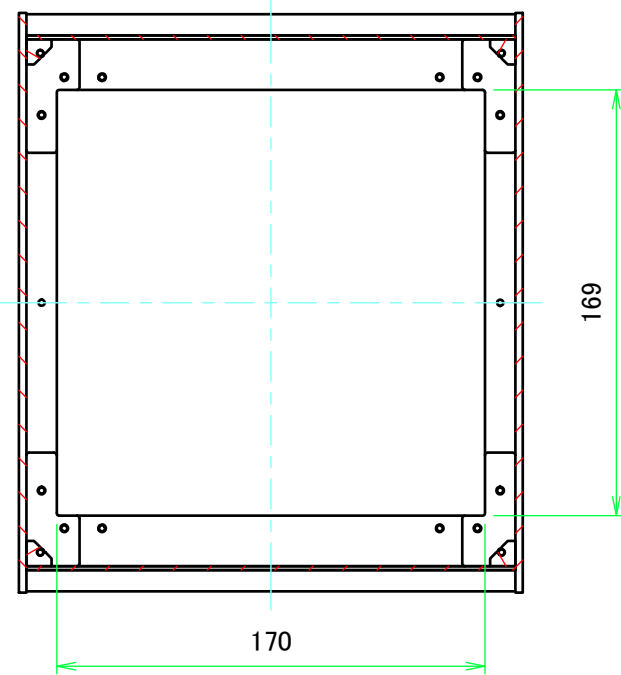
B-B (1:3)
