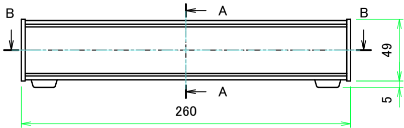
A view
