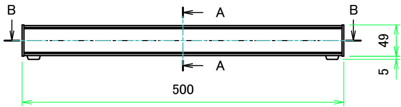
A view
