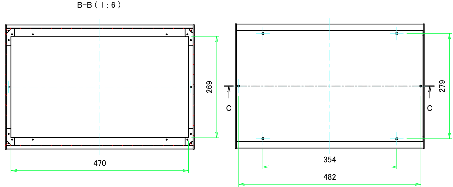
E view
