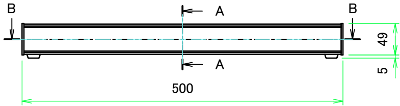
A view
