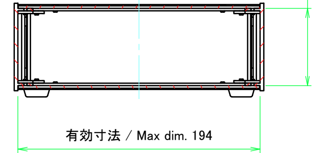
C-C (1:3)
