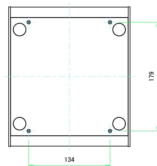
F view
