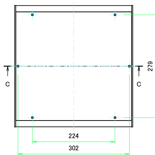
E view
