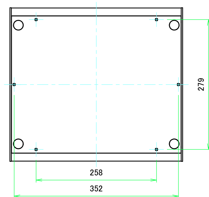
F view
