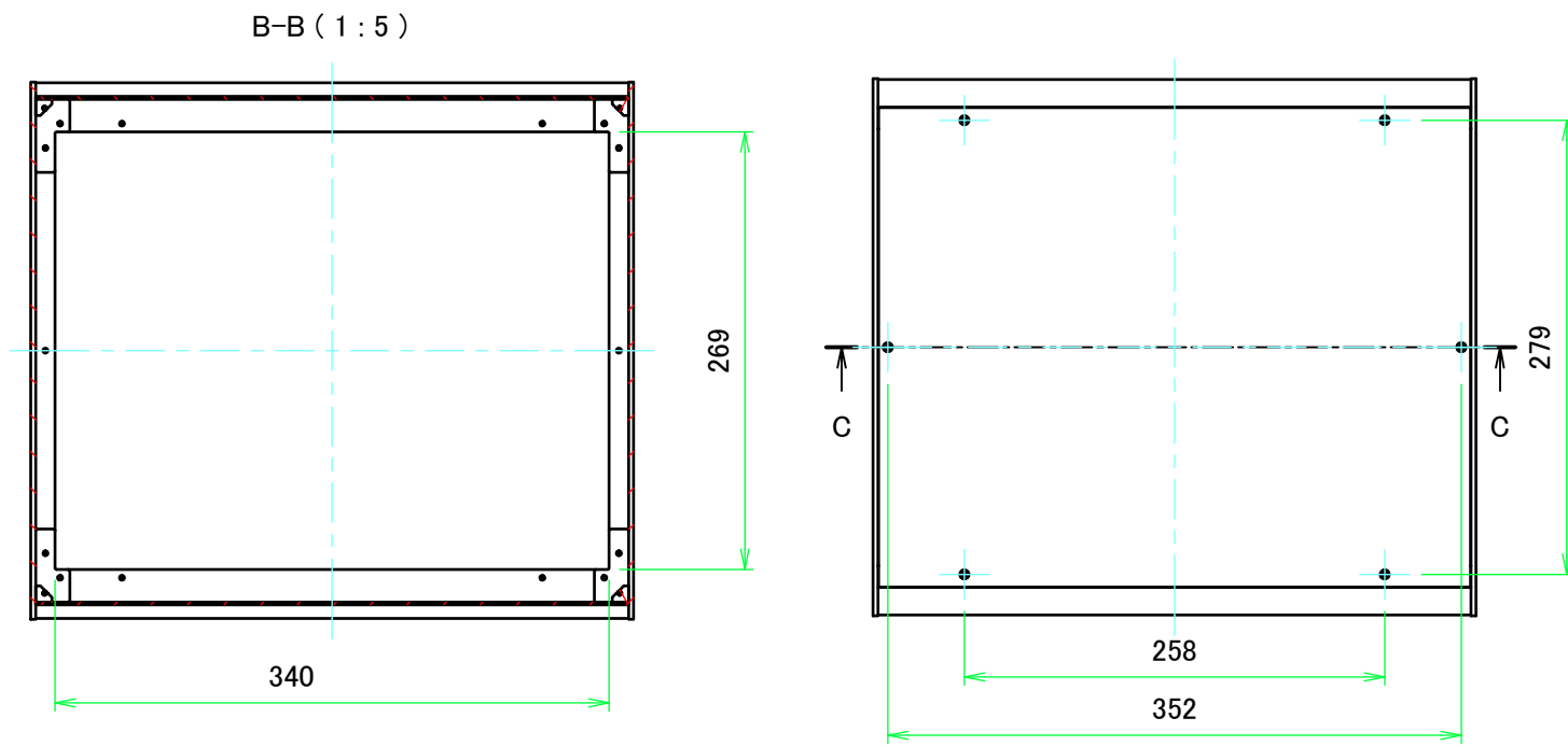
D view
