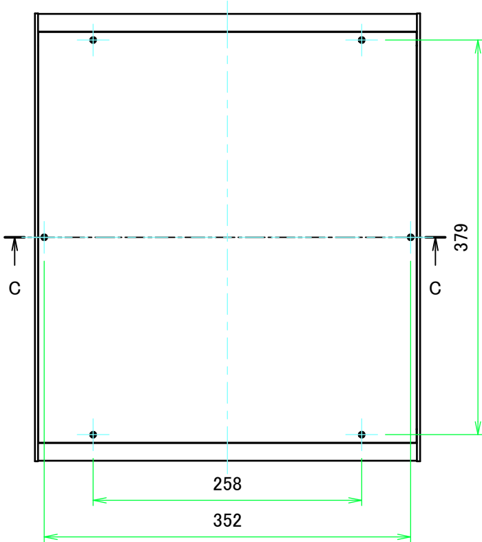
A view
