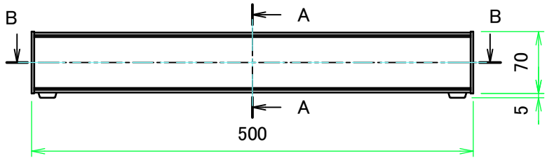
A view
