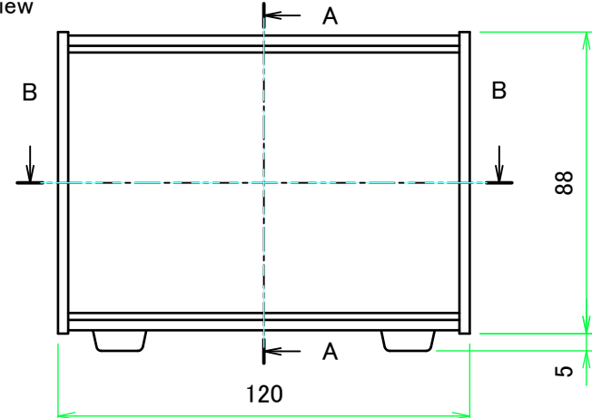
F view
