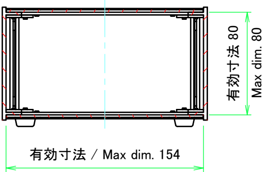
C-C (1:3)
