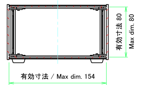
C-C (1:3)
