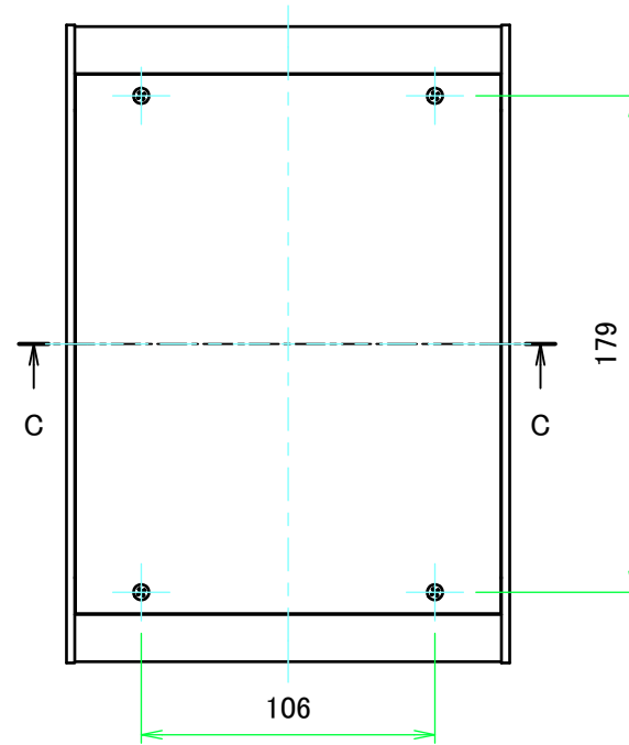
E view
