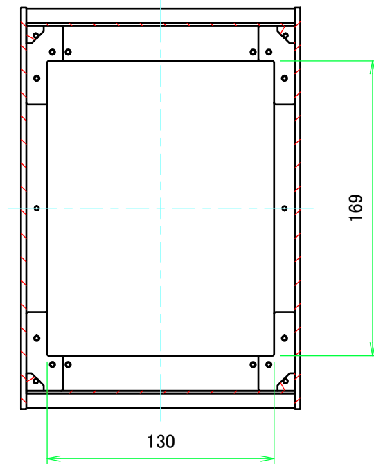
B-B (1:3)
