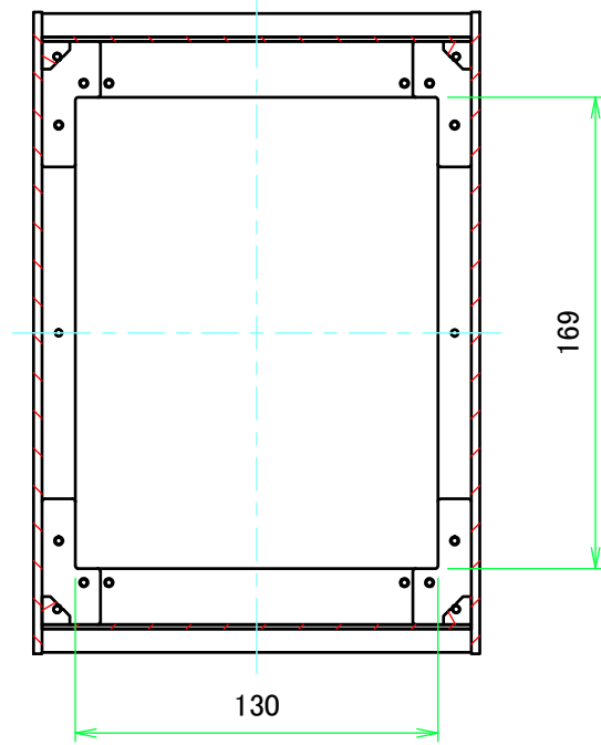
B-B (1:3)
