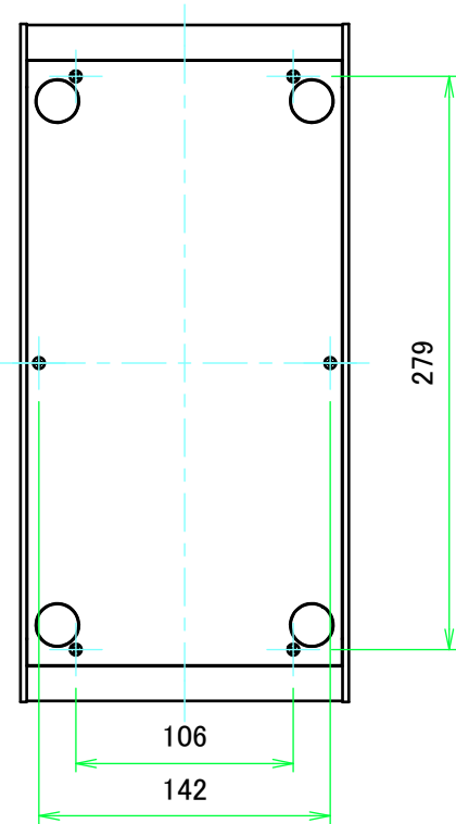
F view
