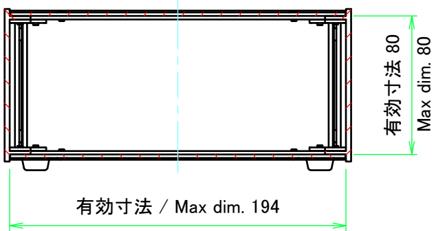
C-C (1:3)
