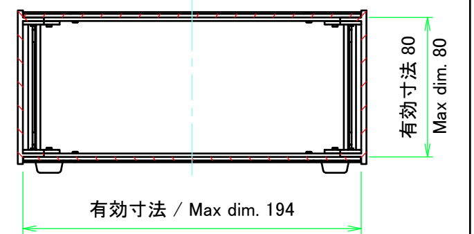
C-C (1:3)
