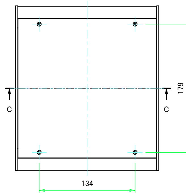
E view
