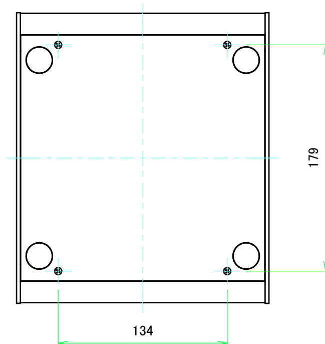
F view
