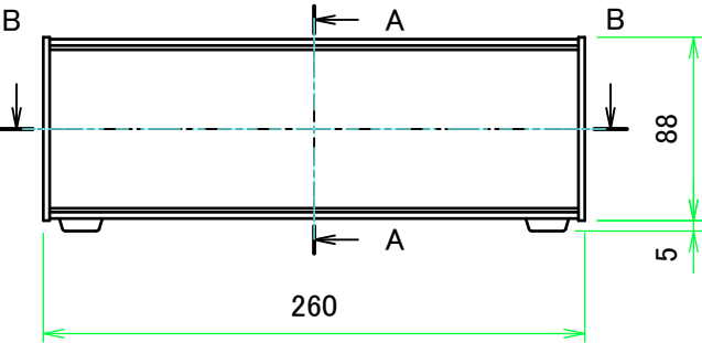
A view
