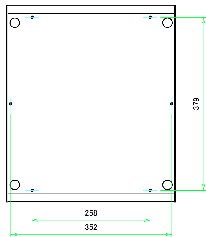
F view
