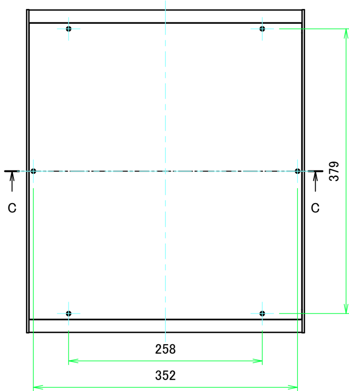
A view
