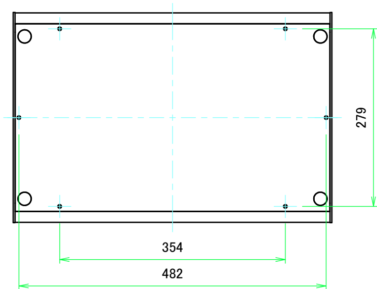
F view
