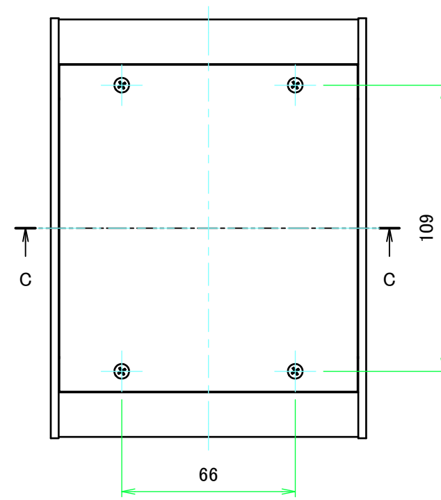
A view
