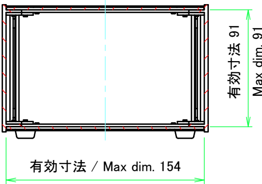
C-C (1:3)
