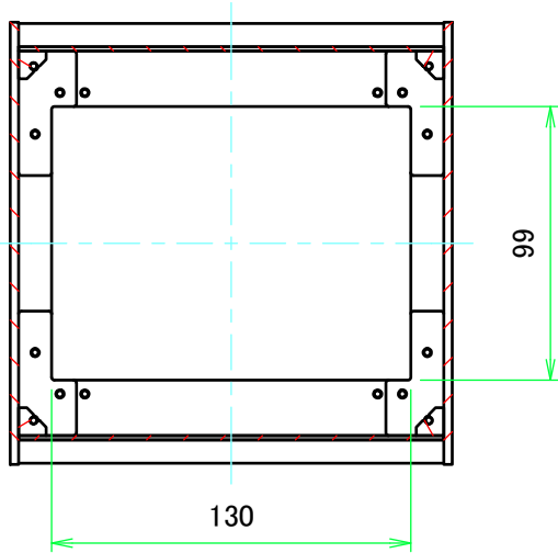
B-B (1:3)
