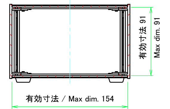
C-C (1:3)
