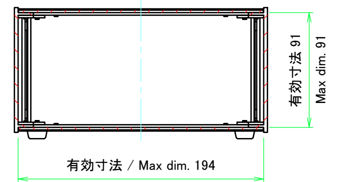
C-C (1:3)
