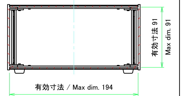
C-C (1:3)
