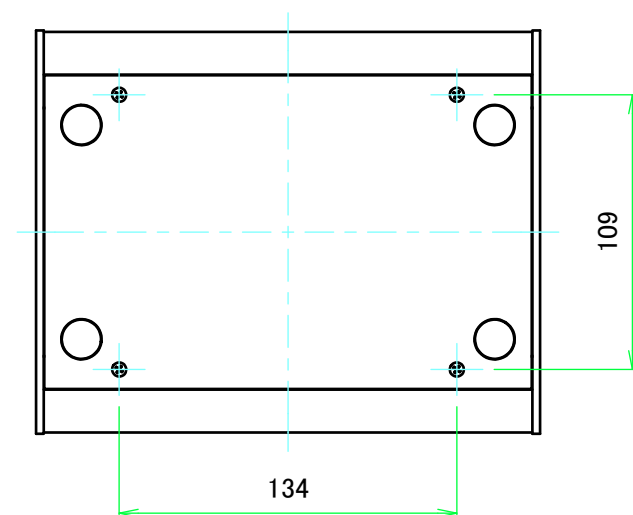
F view
