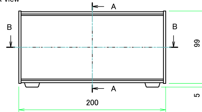
A view
