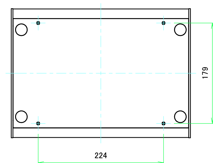
F view
