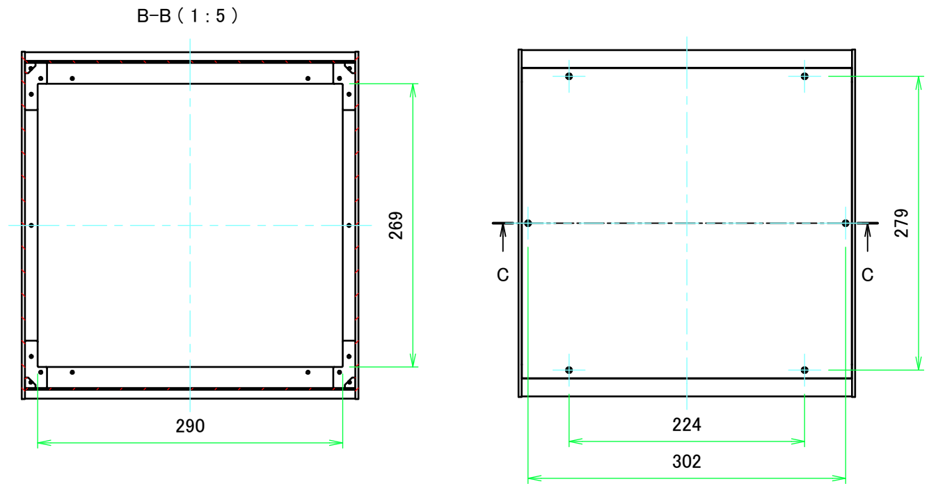
E view
