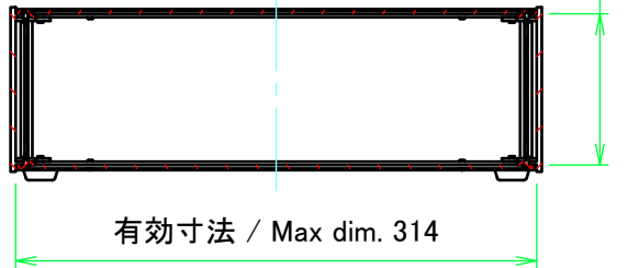
C-C (1:5)
