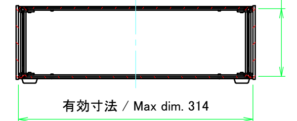
C-C (1:5)
