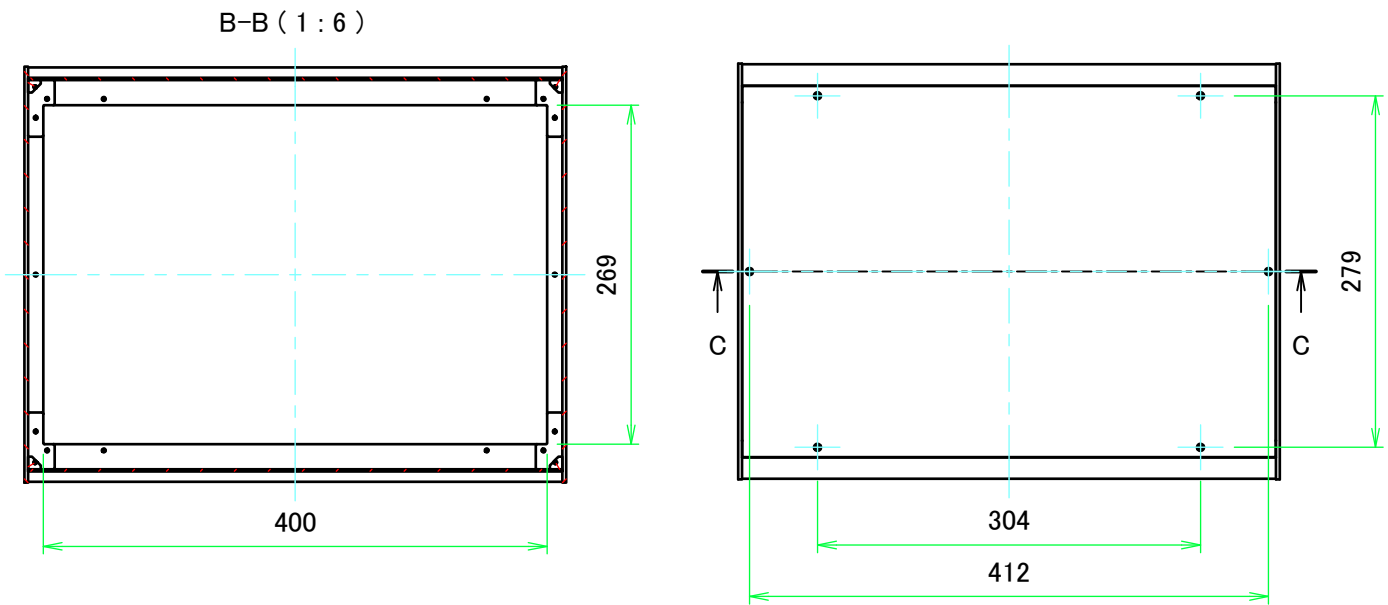
E view
