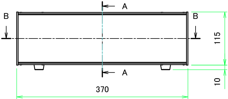
A view
