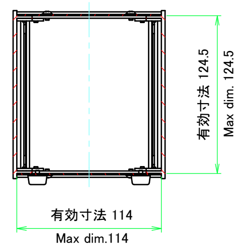
C-C (1:3)
