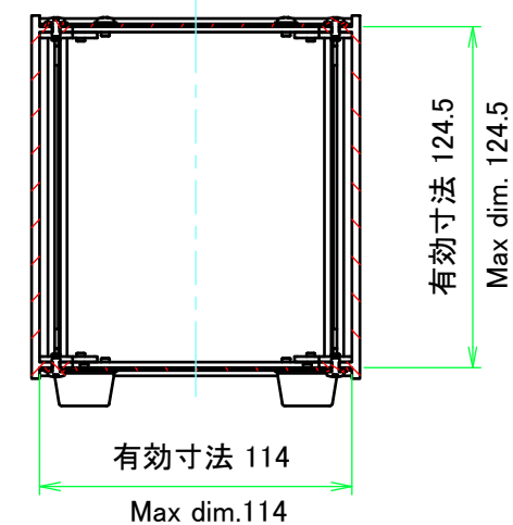
C-C (1:3)
