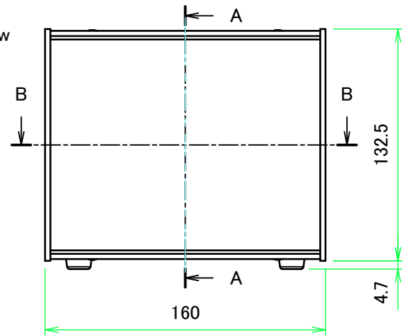
C view
