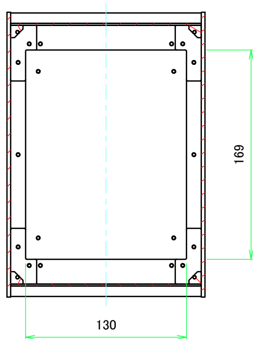
B-B (1:3)
