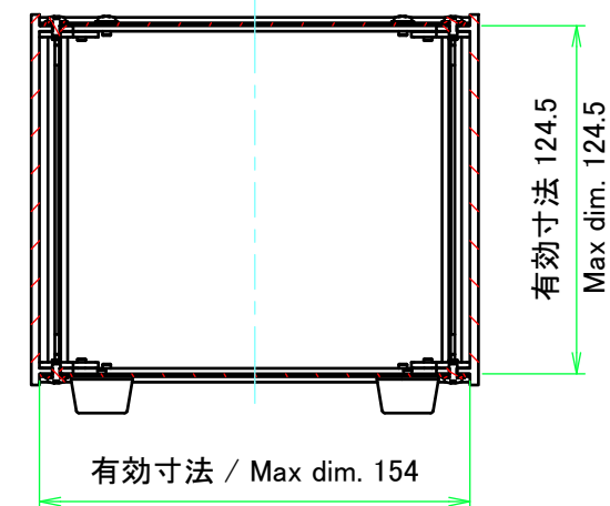
C-C (1:3)
